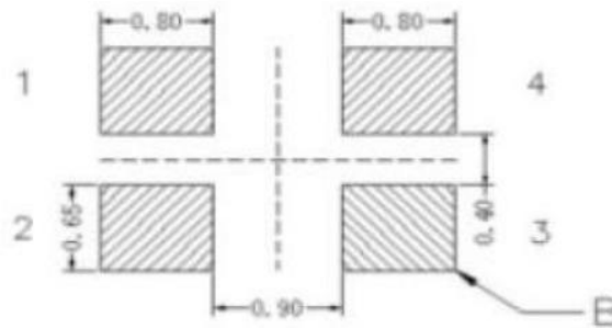
Reference Soldering Pad
