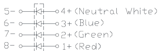
Circuit Diagram
